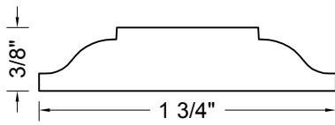
4918 MUL 3/8" x 1-3/4"
