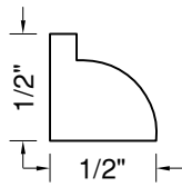
4910 STOP 1/2" x 1/2"
