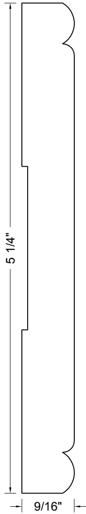
4002 CHB 9/16" x 5-1/4"
