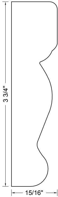
3101 CAP 15/16" x 3-3/4" Plinth For 3001 CA
